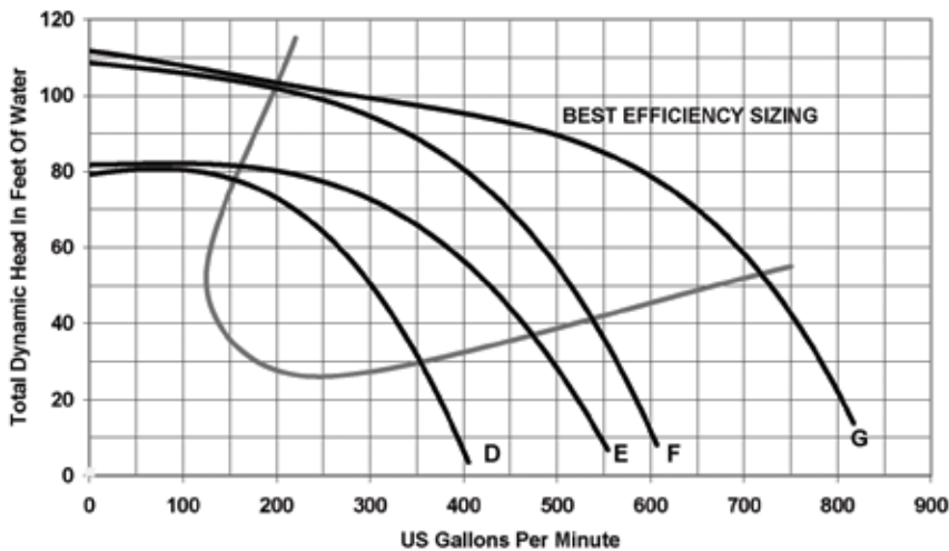
EQK SERIES PERFORMANCE CURVES
