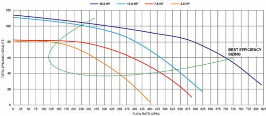
JCP Performance Curves with Strainer
